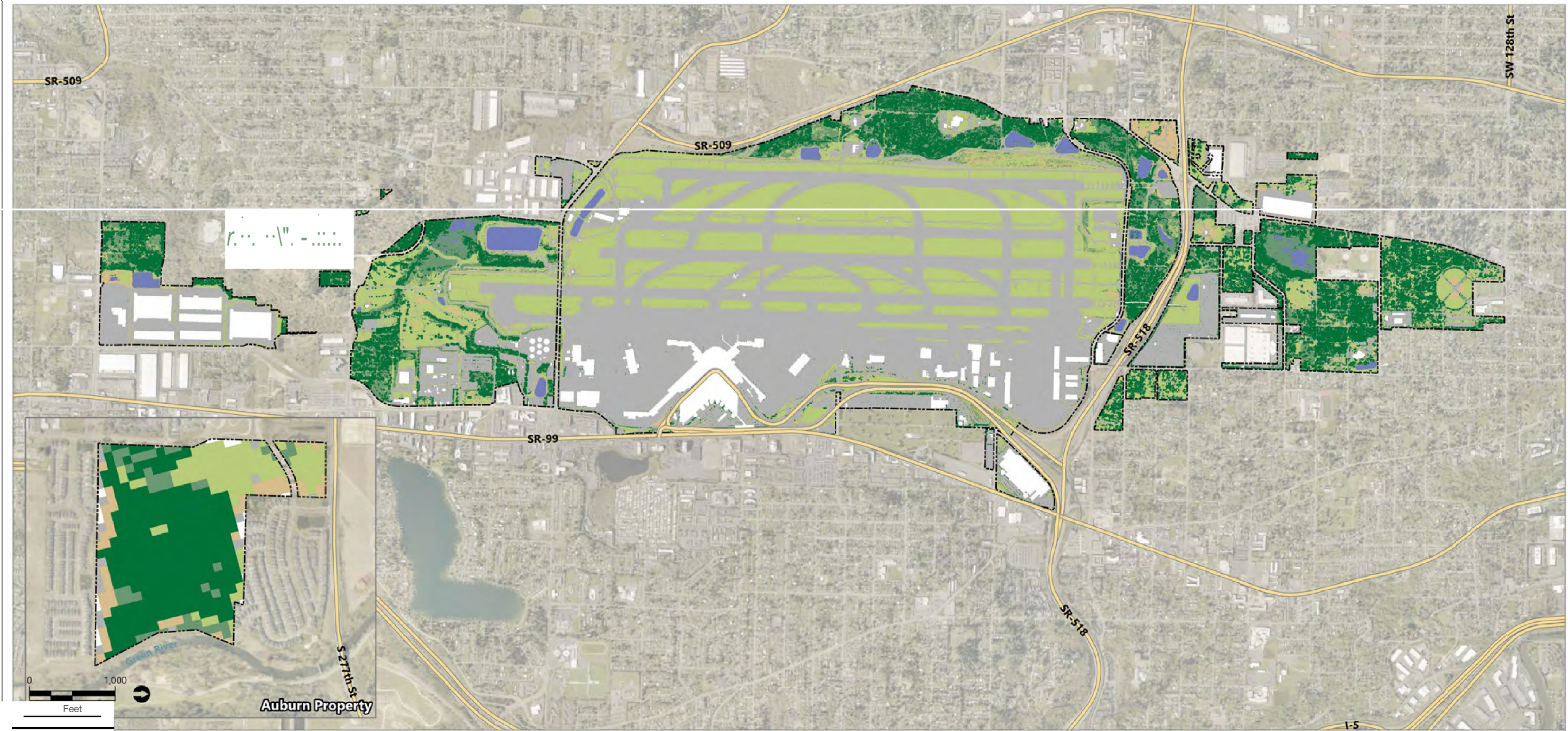
Figure 5 2021 Land Cover
